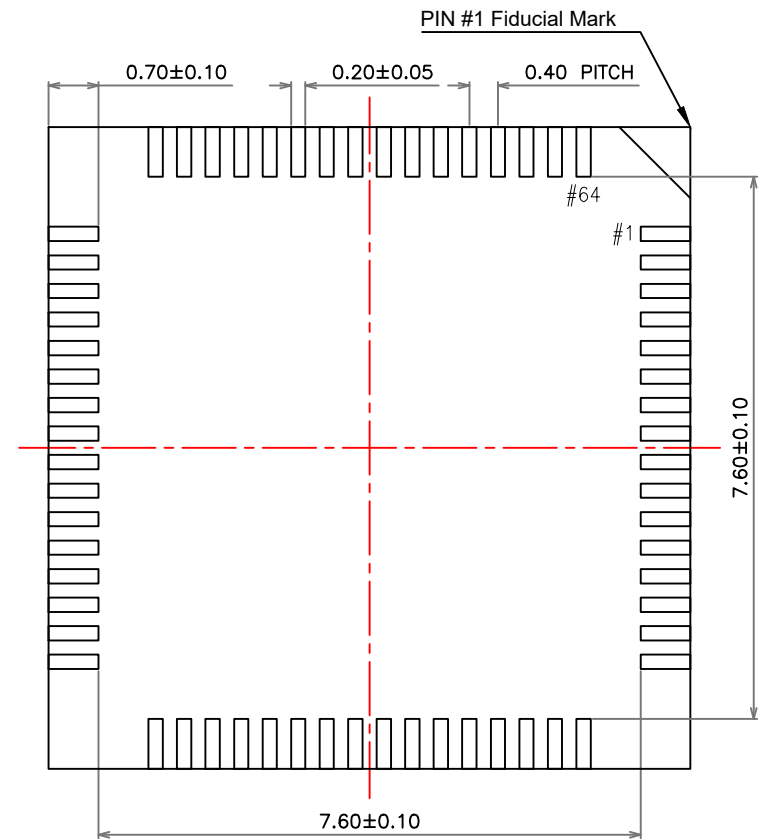
BOTTOM VIEW
